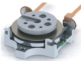
θ axis Stage
