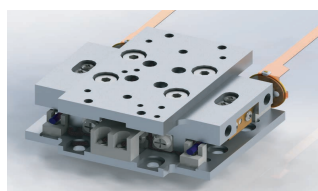
X axis Stage with Cross roller guide
