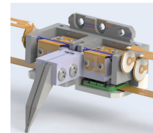
Finger Unit with Encoder
