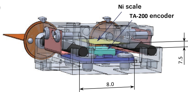
TULA Stage XMDT 50-057 Structure
