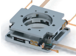
XY axes Hollow Stage
