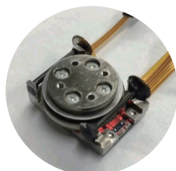
TULA Stage \theta MDT 50-1802 Structure
