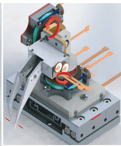
◆X θ 1 θ 2F type (X Stage: 0.1 \mu\text{m} , \theta : 0.005^\circ )
